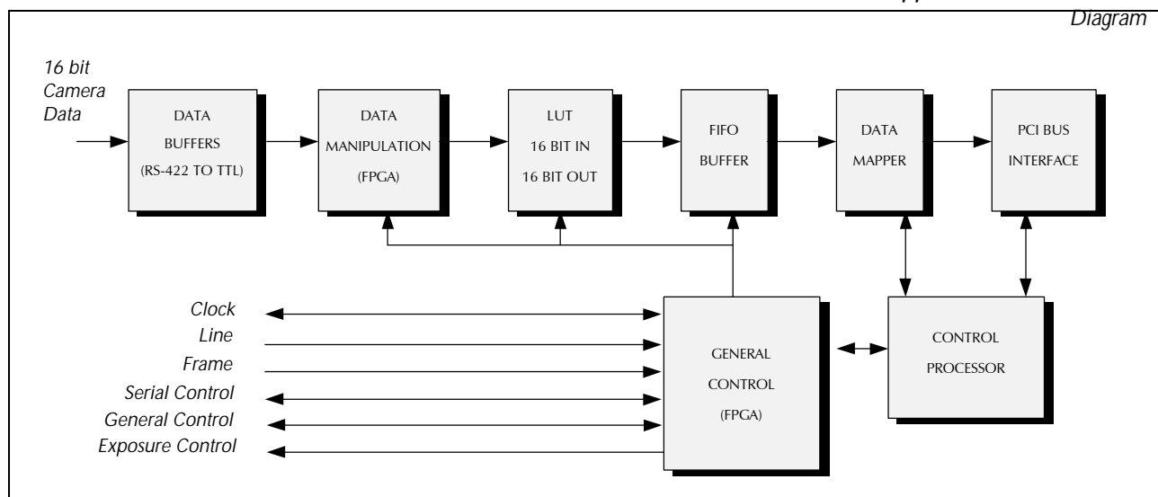
Snapper-PMC-DIG16 Block
